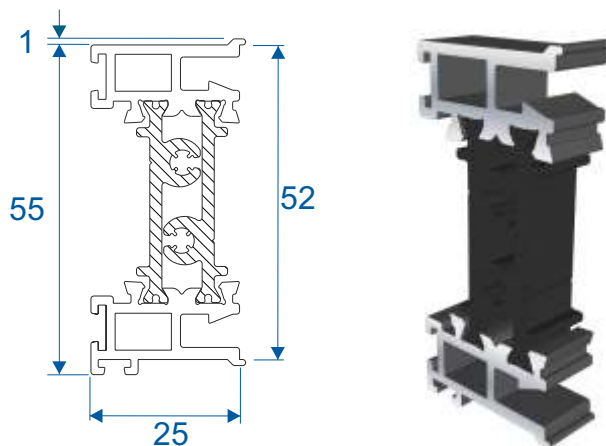
VS024 - Vertical Member
