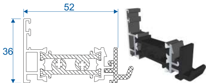
VS021 - Interlock Top Panel
