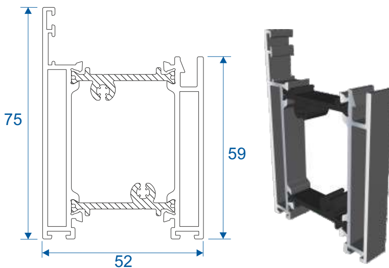
VS022 - Interlock Bottom Panel
