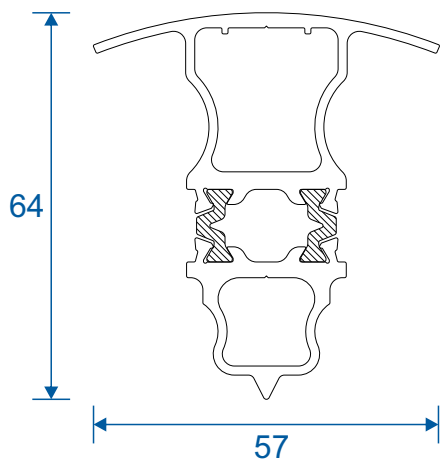
AW717 - 140 to 160° Bay Pole
