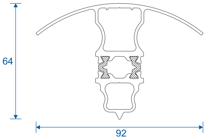
AW716 - 120 to 140° Bay Pole
