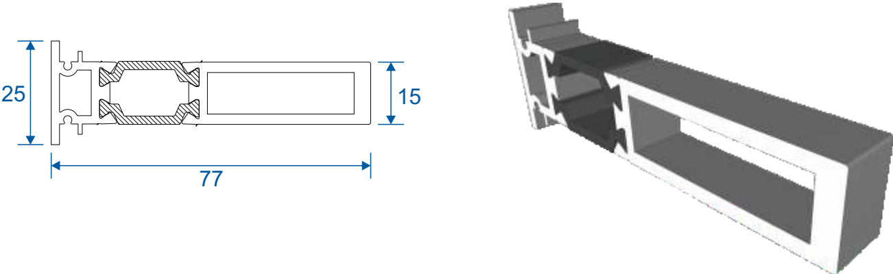
AW702 - 15mm Coupler For 70mm Frame
