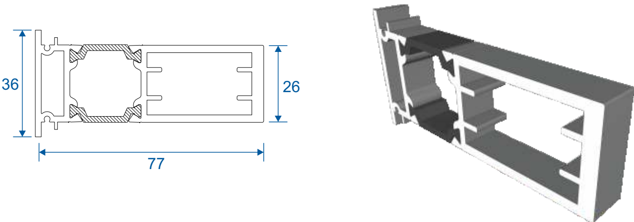
AW705 - 26mm Coupler For 70mm Frame
