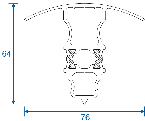
AW717 - 140 to 160° Bay Pole
