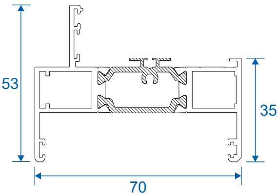
AW622 - 70mm Square Equal Leg
