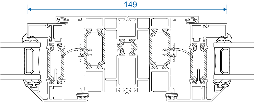
Coupling 58mm Outer Frames - AW710
