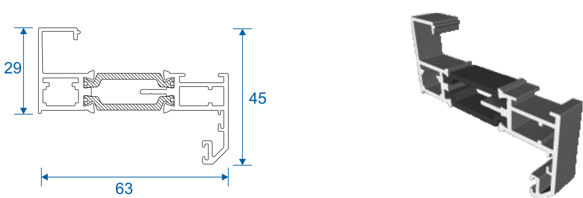
AW690 - Externally Glazed Feature Sash
