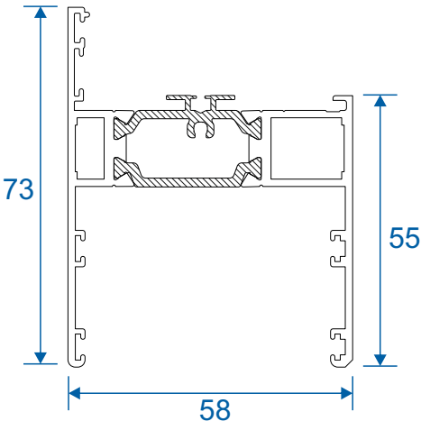
AW608 - 58mm Deep Equal Leg
