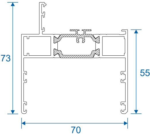
AW623 - 70mm Deep Square Equal Leg
