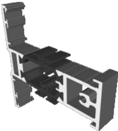
AW631 - 57mm Transom / Mullion
