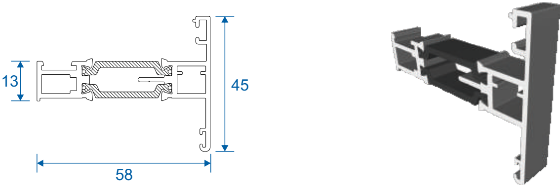
AW686 - Internally Glazed Stepped Sash
