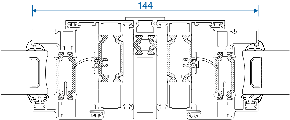
Coupling 58mm Outer Frames - AW703
