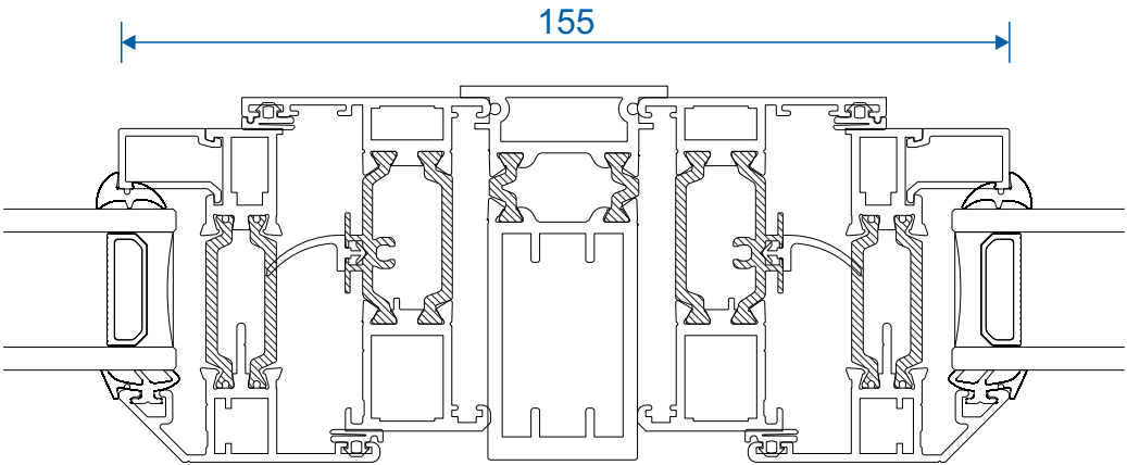
Coupling 58mm Outer Frames - AW706
