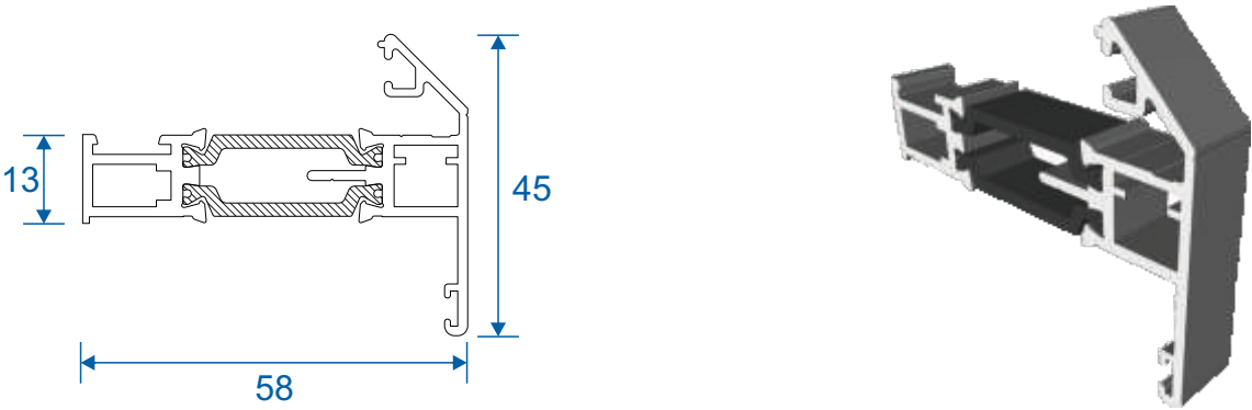
AW690 - Externally Glazed Feature Sash
