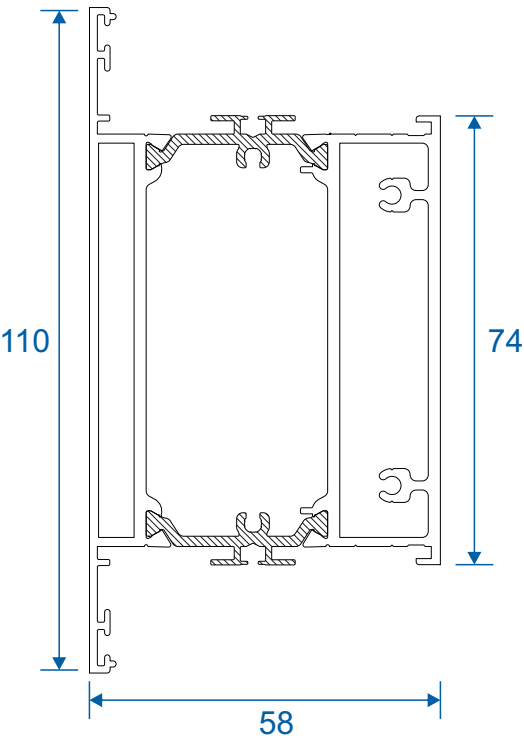
AW635 - 110mm Midrail
