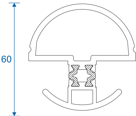
AW712 - 60mm Circular Bay Pole
