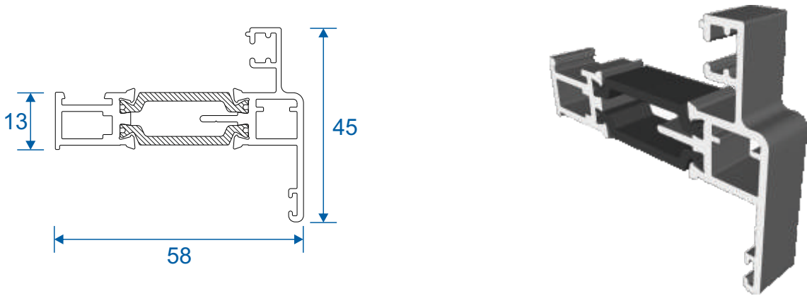
AW614 - Internally Glazed Chamfered Sash
