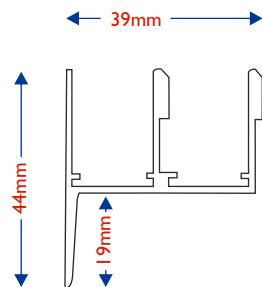
Horizontal / Vertical Sliders Economy Odd Leg Fix
