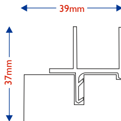
Lift Out SF1 Face Fix Subframe
