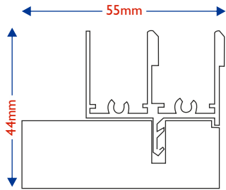
Horizontal / Vertical Sliders SF3 Reveal Fix Subframe
