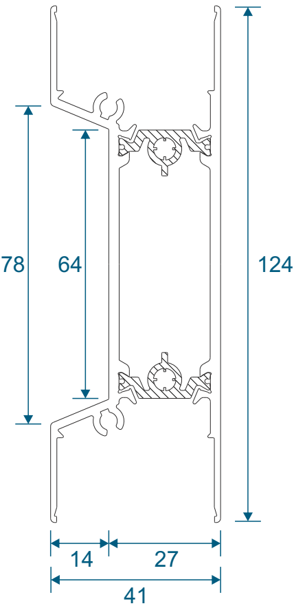
GSL1130 - Letter Plate
