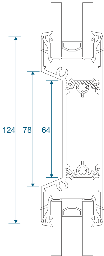
124mm Letter Plate
