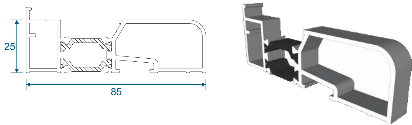
ETC451 - 85mm Cill
