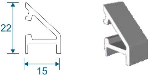
VL72 - Weather Drip
