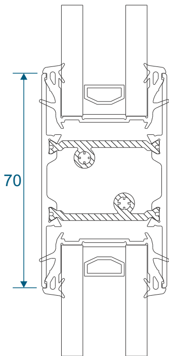
70mm
