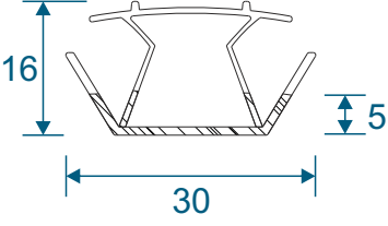
GSL051 - Channel Infill
