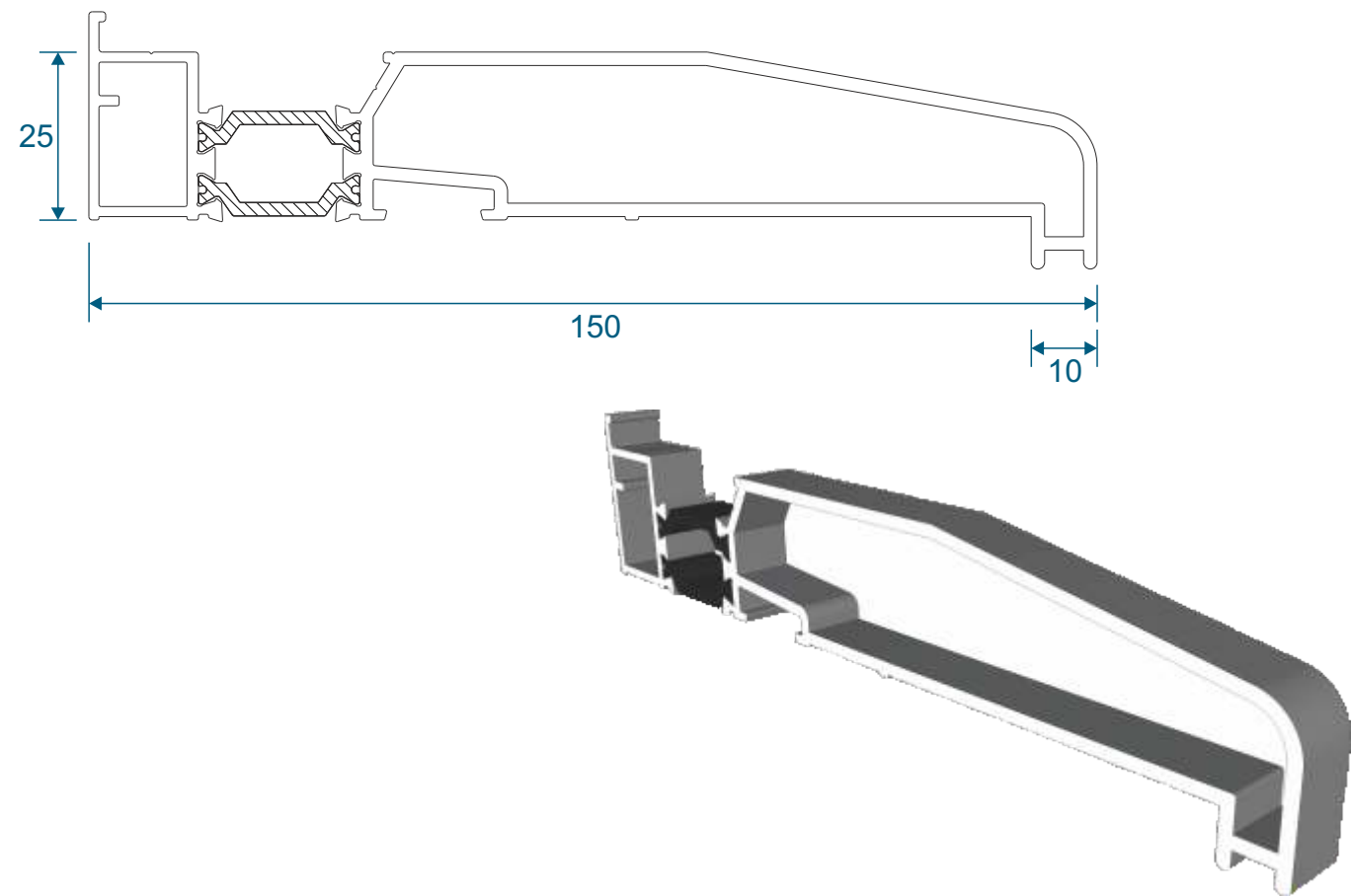
ETC457 - 150mm Cill
