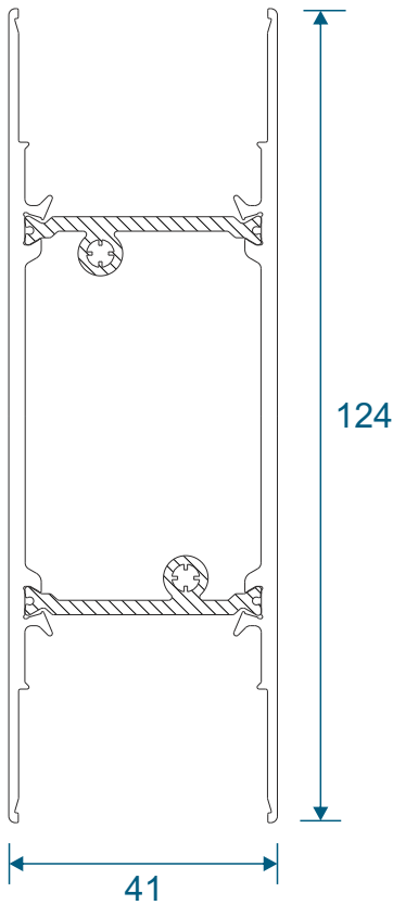
GSL1131 - 124mm
