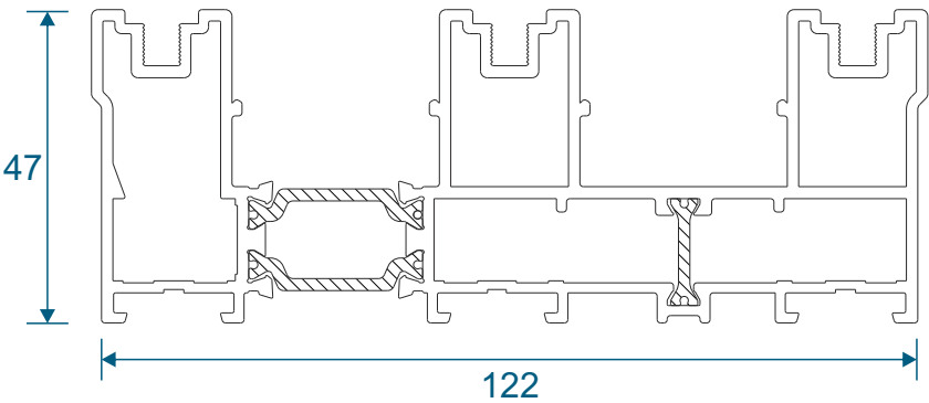
GSL1012 - Three Track
