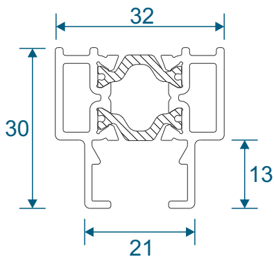
GSL040 - Meeting Stile Adapter
