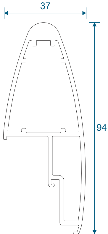
GSL1330 - Heavy Duty
