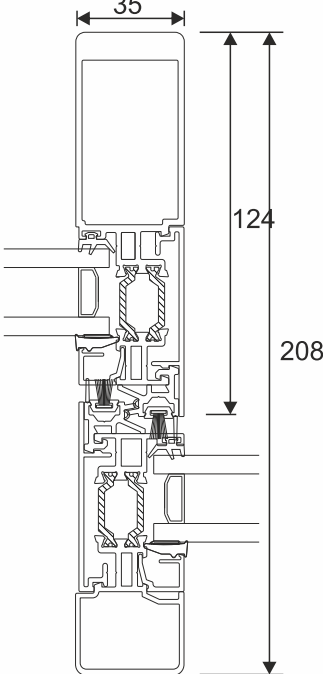
Slim Heavy Duty Interlock N/A for 3 panels
