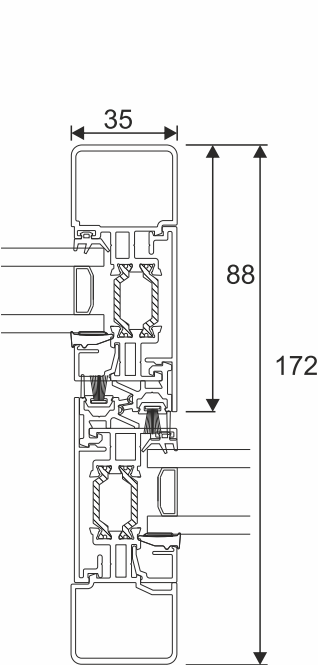
Slim Medium Duty Interlock N/A for 3 panels
