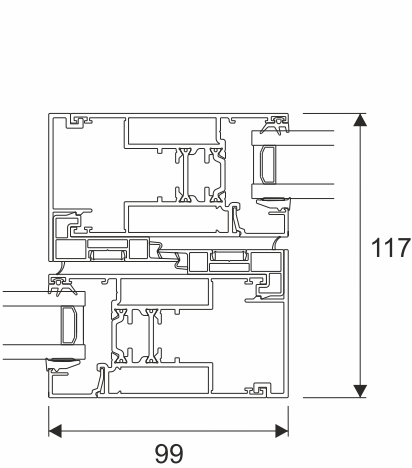
Standard Interlock
