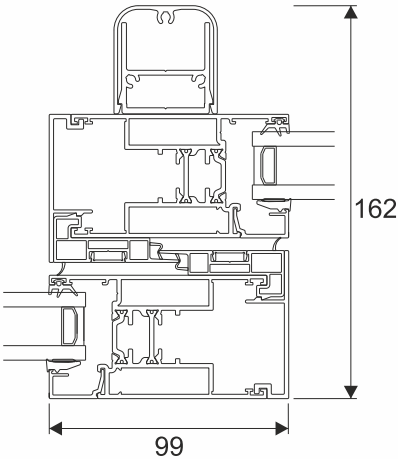
Single Heavy Duty Interlock
