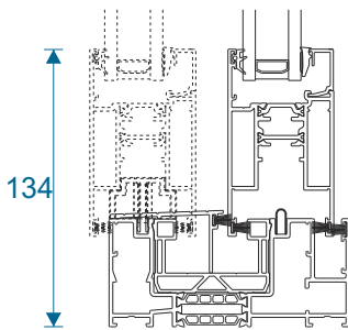
Threshold - No Cill
