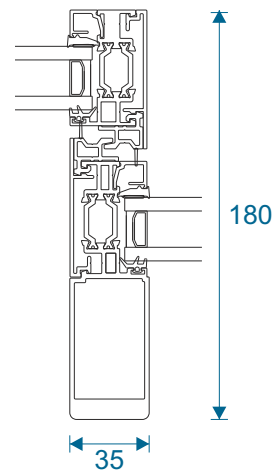
Slim Reinforced Interlock
