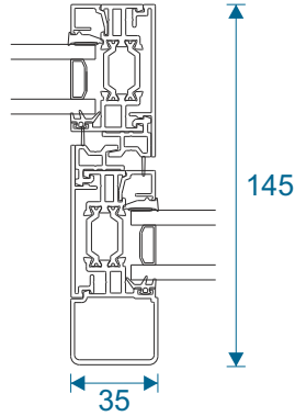
Slim Reinforced Interlock
