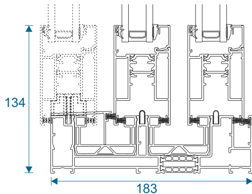
Three Track Threshold With no Cill
