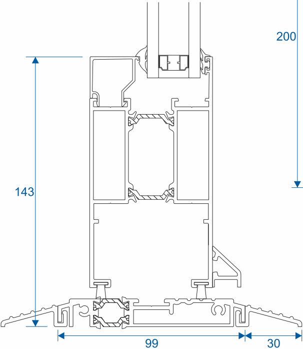
Threshold
