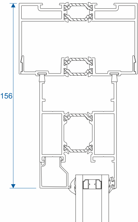
Head
