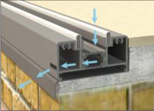
Standard Threshold (Open Out)
