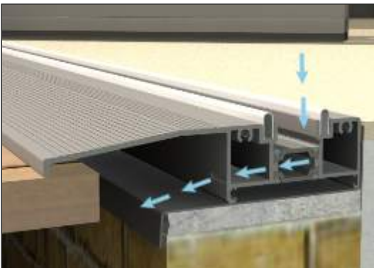
Duration Threshold (With Ramp)
