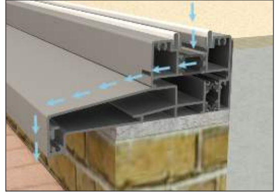
Standard Threshold With Cill (Open Out)
