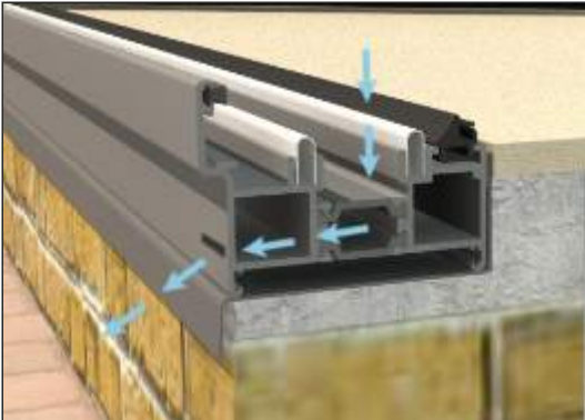
Standard Threshold (Open In)
