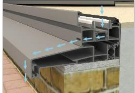
Standard Threshold With Cill (Open In)
