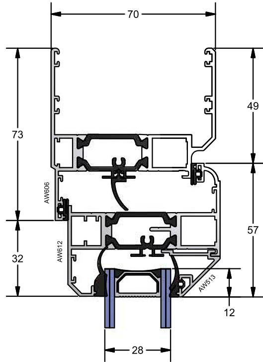
Deep Equal Leg Frame Detail
