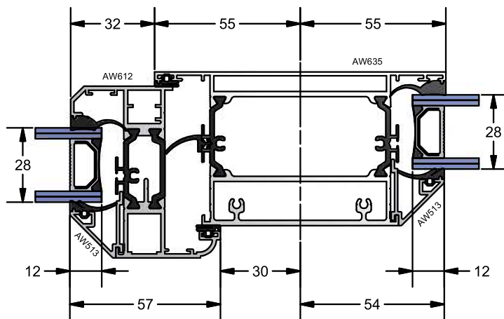
AW 635 Window Midrail Detail
