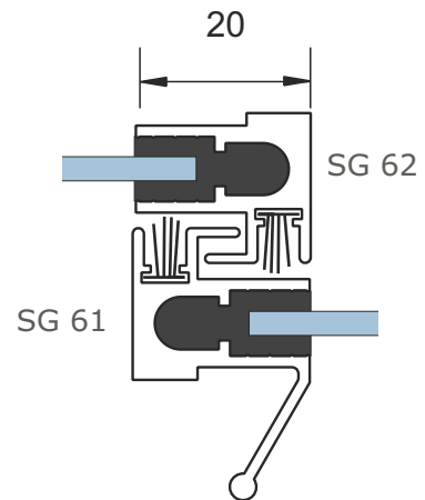
B - 1st Interlock
