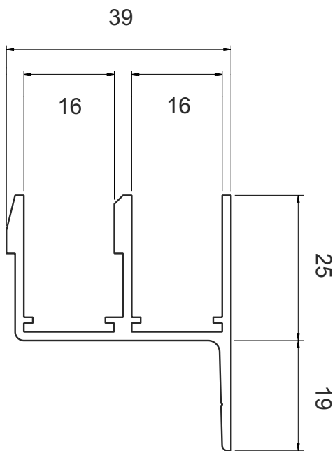
SG 92 Odd Leg Outerframe with screw ports
