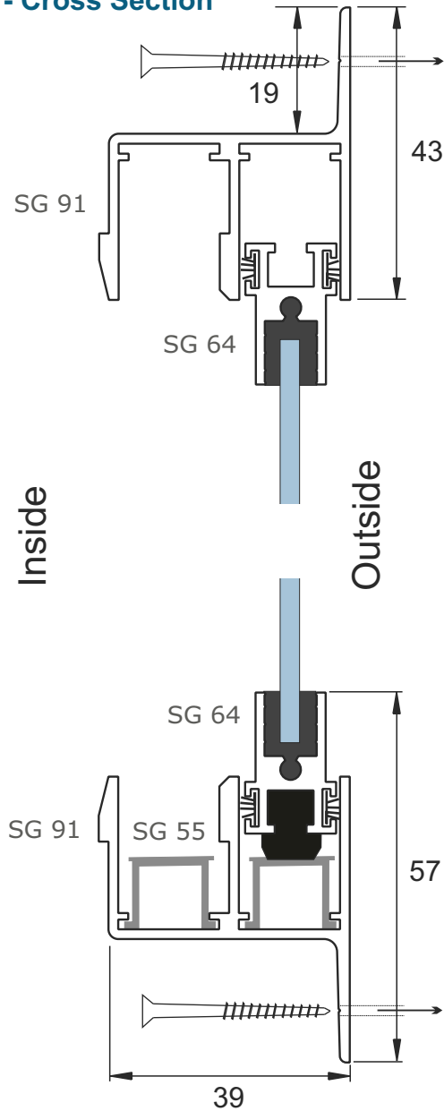
G - Cross Section
