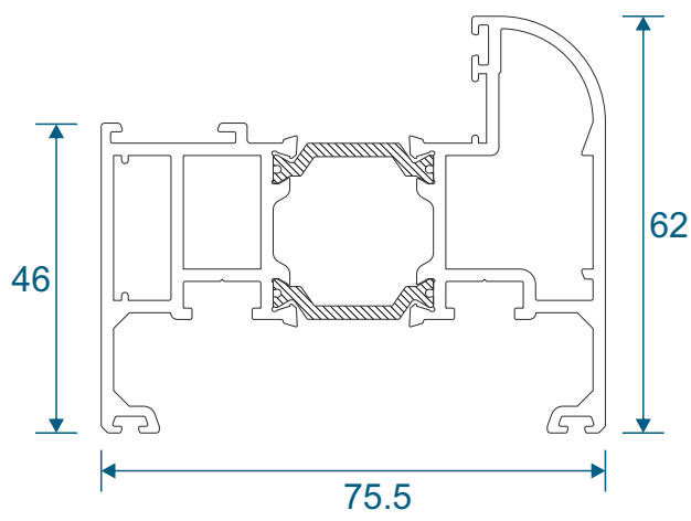
DV526 - Radius Sash
