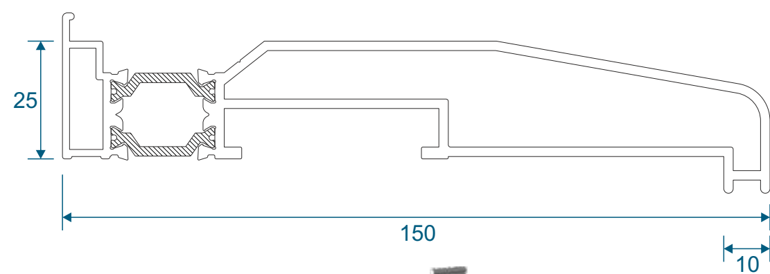
ETC157 - 150mm Cill
