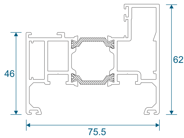
DV528 - Square Sash
