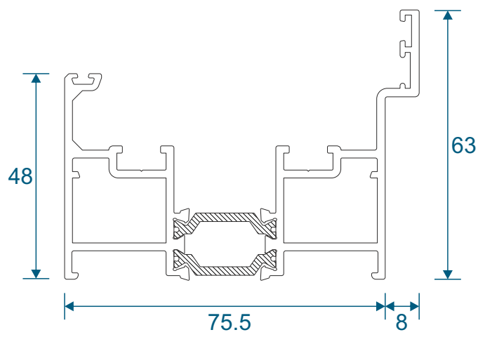
DV510 - Outerframe / Threshold
