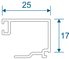
DV160 - 24mm Square Bead
