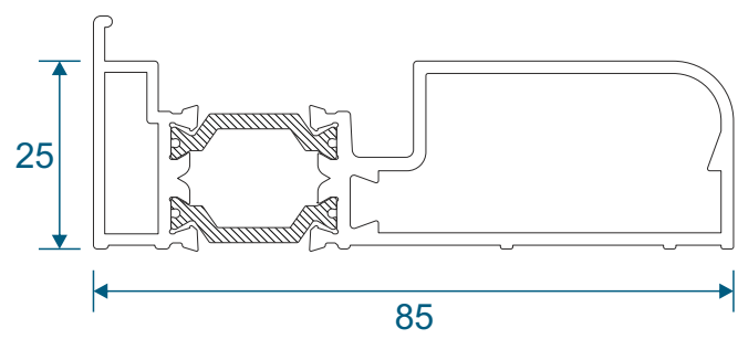
ETC178 - 85mm Cill
