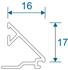
DV64 - 32mm Chamfer Bead
