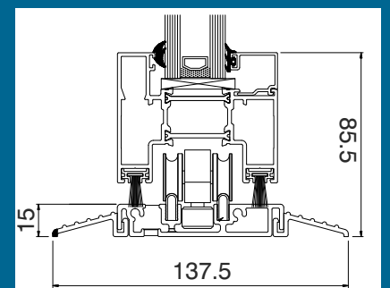
15mm Ramped Low Threshold
