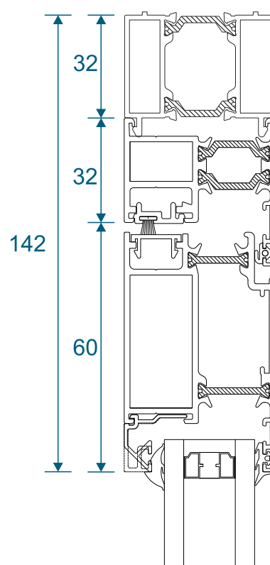
32mm Extension On ETD010
