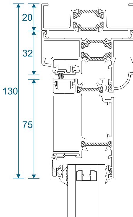
20mm Extension On ETD014
