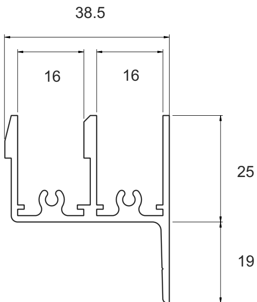
SG 92 Odd Leg Outerframe with screw ports
