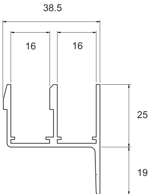
SG 91 Odd Leg Outerframe no screw ports
