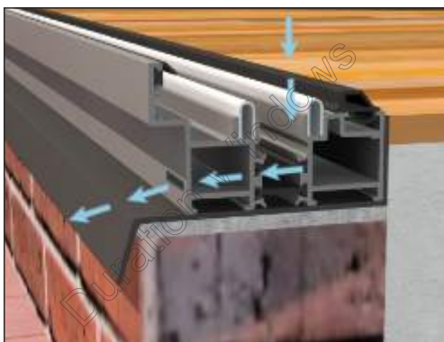
Standard Threshold (Open In)
